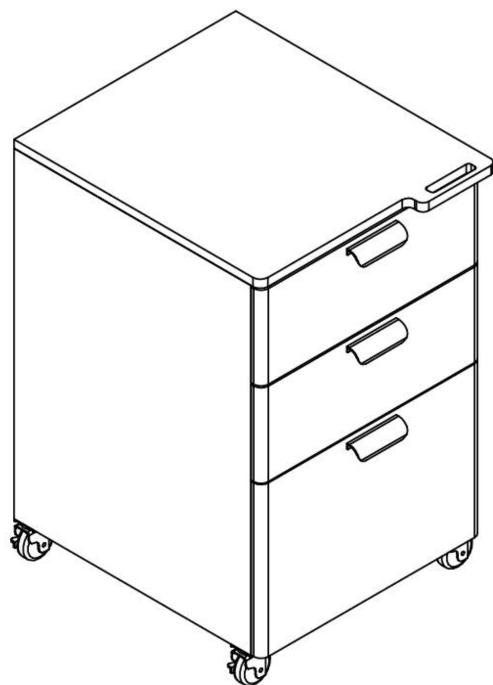
V9 3 drawer mobile cabinet single piece drawing
